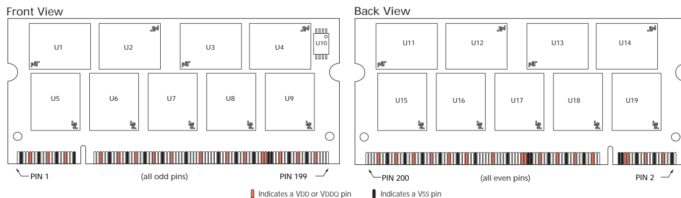
Figure 2: Module Layout
