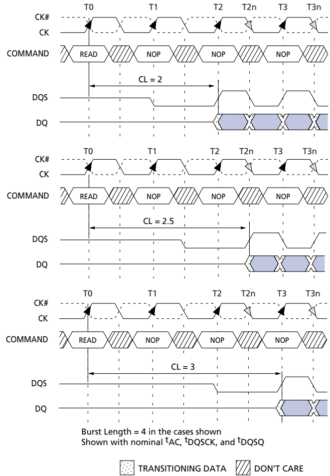
Figure 6: CAS Latency Diagram
