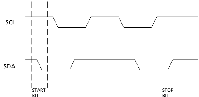
Figure 11: Definition of Start and Stop
