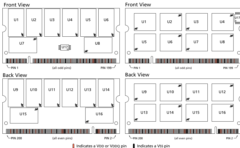
Figure 2: Module Layout
