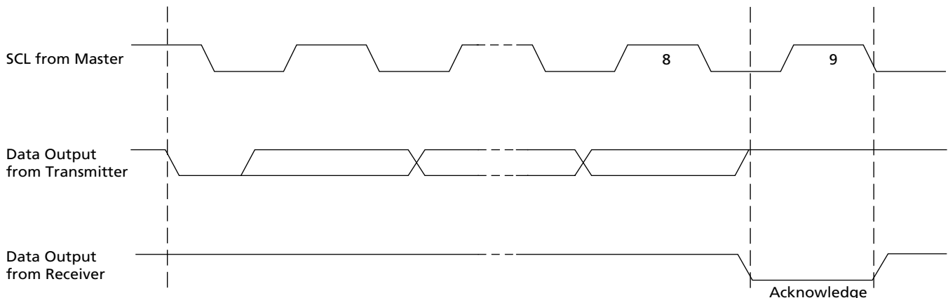
Figure 12: Acknowledge Response From Receiver
