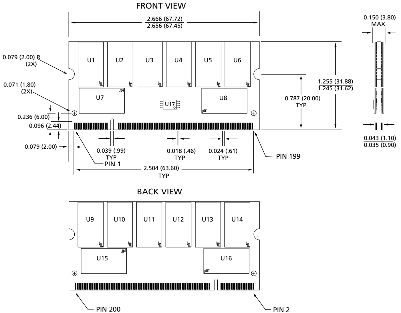
Figure 14: 200-PIN SODIMM Dimensions – 512MB
