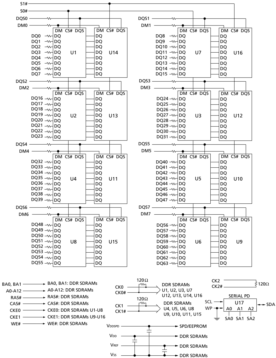
Figure 3: Functional Block Diagram – 512MB
