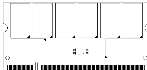
Figure 1: 200-Pin SODIMM (MO-224)
