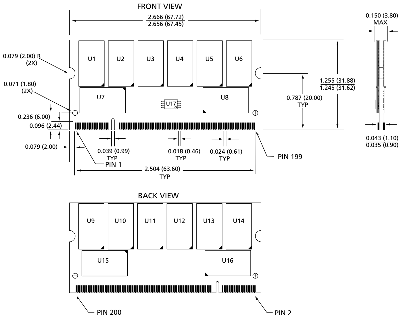
Figure 14: 200-PIN SODIMM Dimensions
