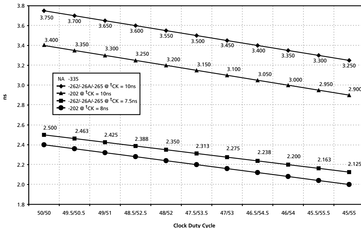
Figure 7: Derating Data Valid Window
