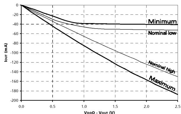
Figure 9: Pull-Up Characteristics
