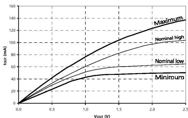
Figure 8: Pull-Down Characteristics
