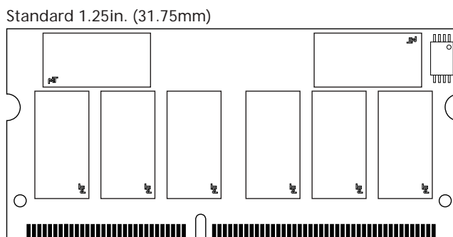
Figure 1: 144-Pin SODIMM (MO-190)
