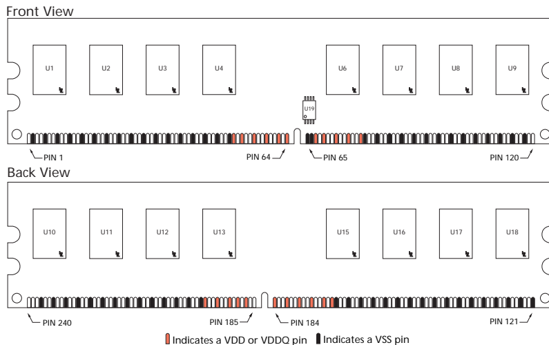
Figure 2: Pin Locations
