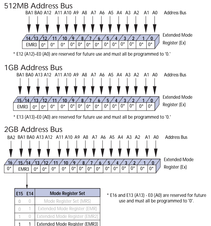
Figure 11: Extended Mode Register 3 (EMR3) Definition
