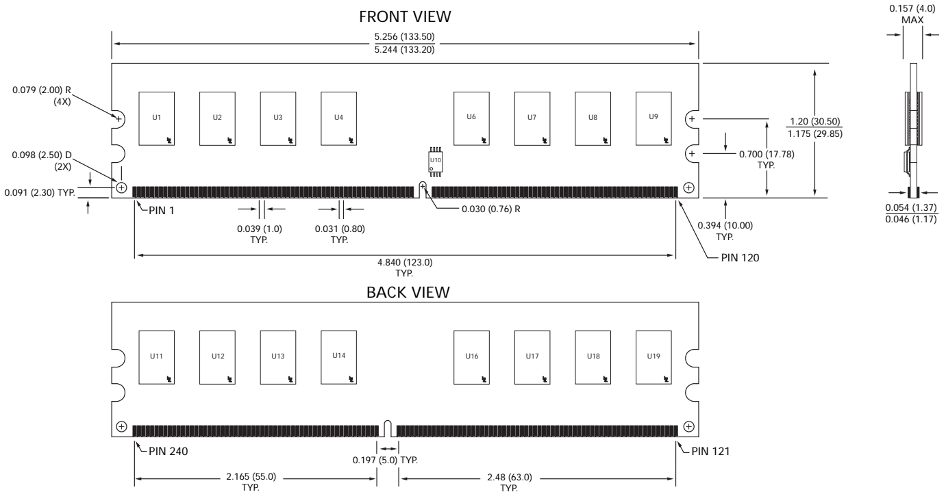
Figure 16: 240-pin DIMM DDR2 Module Dimensions
