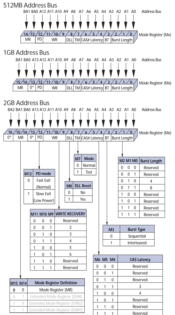
Figure 5: Mode Register (MR) Definition
