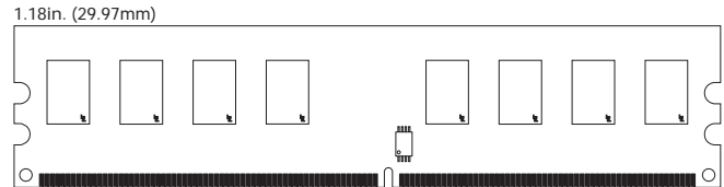
Figure 1: 240-Pin DIMM (MO-237 R/C “B”)
