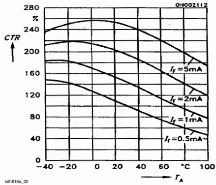
Fig. 4 Current Transfer Ratio (typ.)
