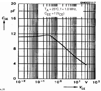
Fig. 7 Transistor Capacitance
