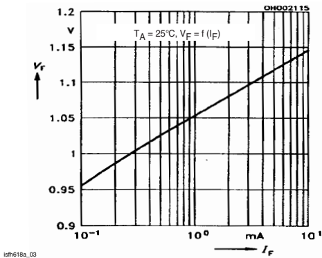
Fig. 5 Diode Forward Voltage (typ.)
