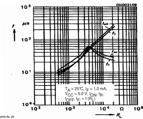
Fig. 11 Switching times (typ.)
