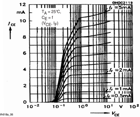
Fig. 8 Output Characteristics
