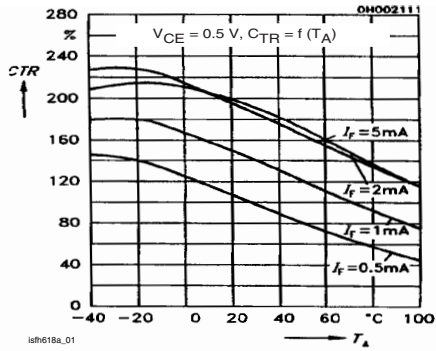
Fig. 3 Current Transfer Ratio (typ.)
