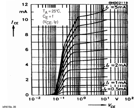
Figure 9. Output Characteristics
