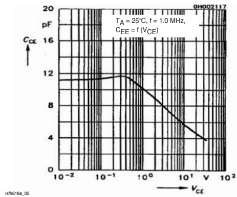
Figure 8. Transistor Capacitance
