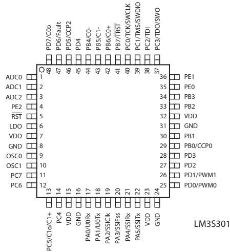
Figure 16-1. Pin Connection Diagram
