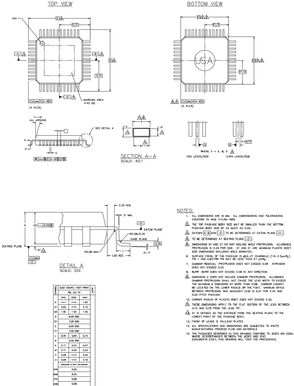
Figure 20-1. 48-Pin LQFP Package
