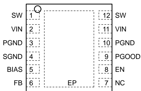
12-Pin 3mm x 3mm MFL (ML)
