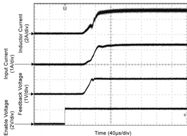
Start-Up Waveforms
