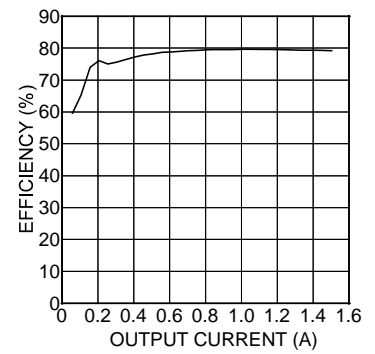
5V IN to 1.5V O Efficiency
