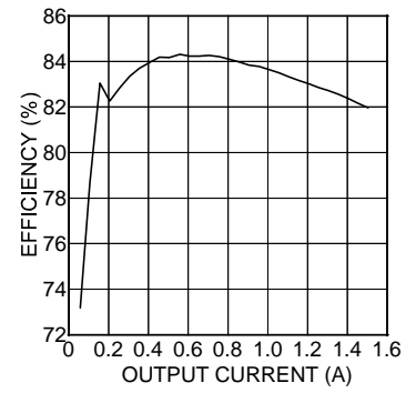
5V IN to 3.3V O Efficiency
