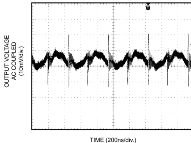
Output Ripple
