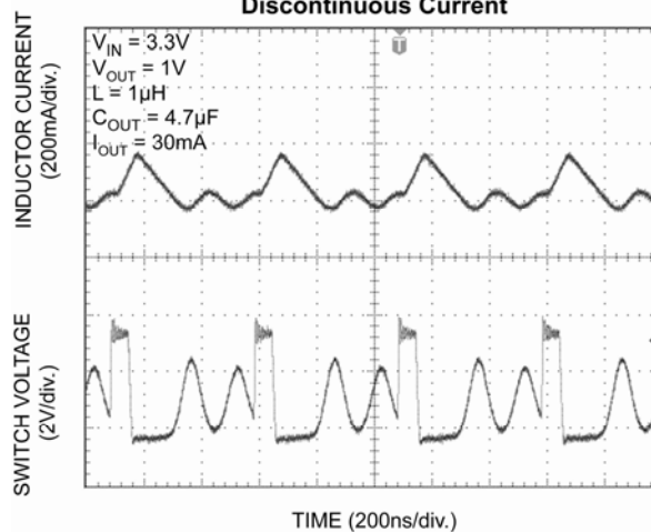
Discontinuous Current
