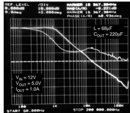
Full-Load Stability Phase Margin = 69°
