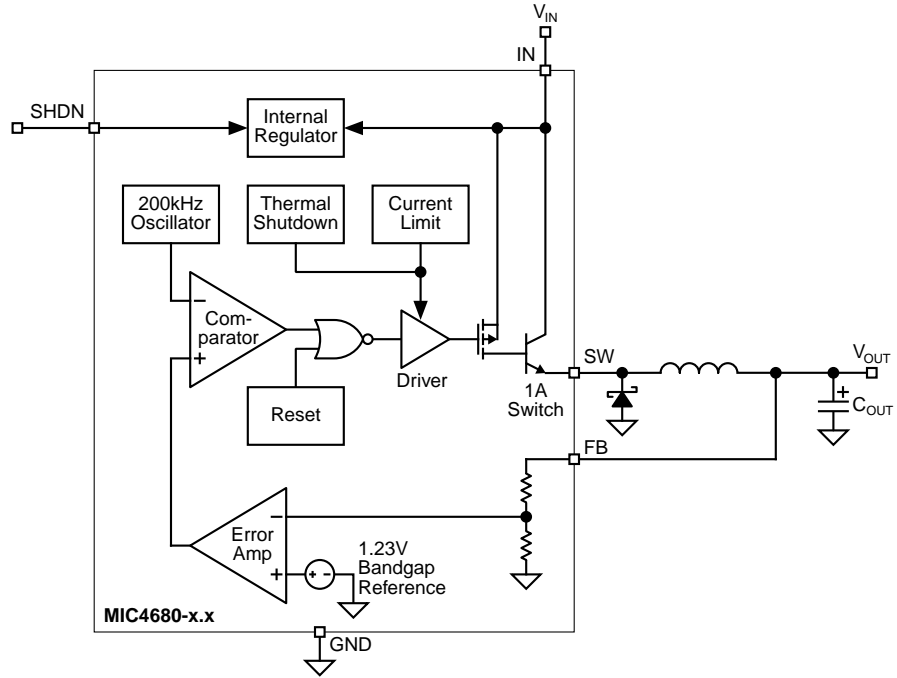
Fixed Regulator
