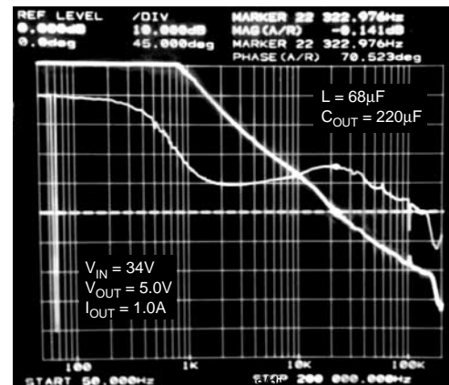
Full-Load Stability Phase Margin = 71°
