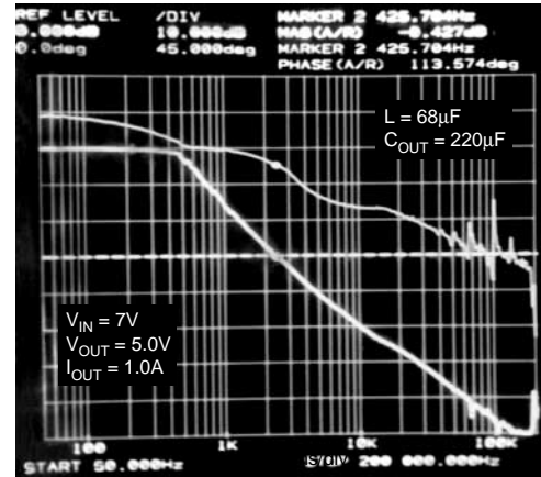
Full-Load Stability Phase Margin = 114°
