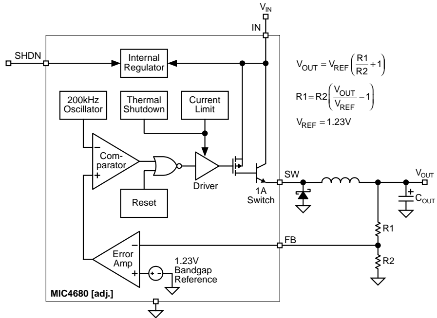
Adjustable Regulator
