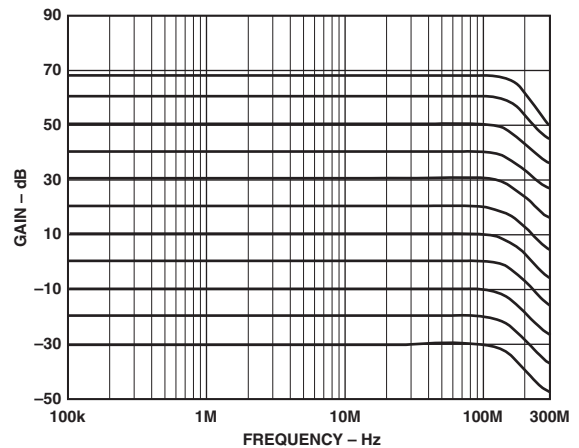
Figure 1. AC Response over the Extended Gain Range
