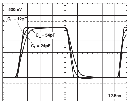
TPC 33. Transient Response vs. for Various Load Capacitances, G = 25\text{ dB}
