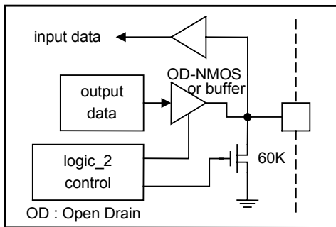
Input/Output IOB port : IOB2 - 0
