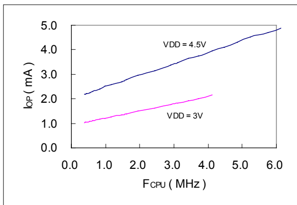
4. Operating current vs. Frequency vs. VDD
