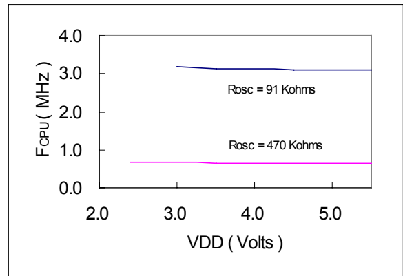
3. Frequency vs. VDD
