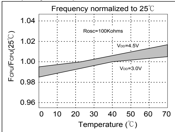
2. Frequency vs. Temperature
