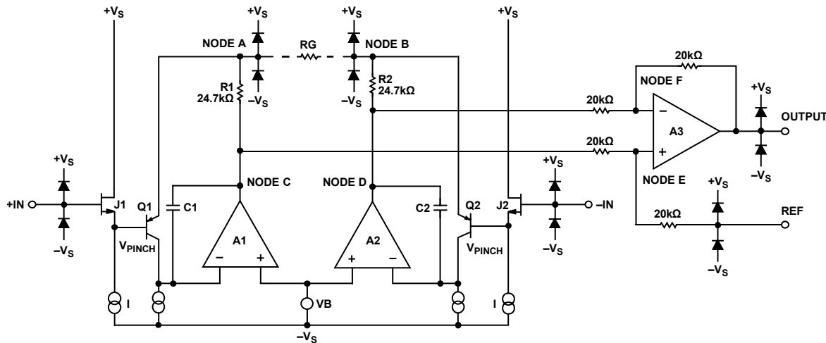
Figure 52. Simplified Schematic
