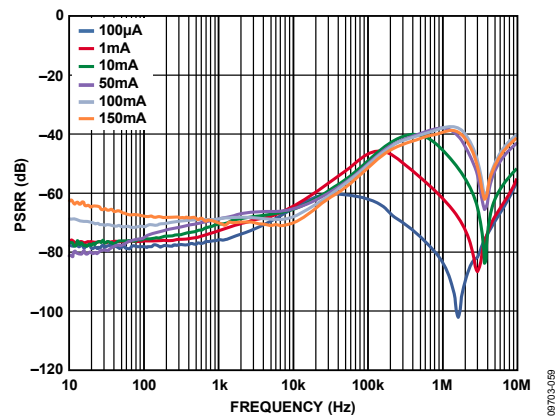
Figure 43. LDO PSRR Across Output Load, V_{IN3} = 5.0 V , V_{OUT3} = 2.8 V
