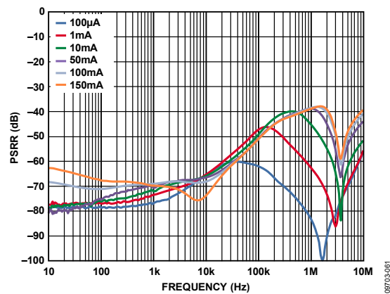
Figure 44. LDO PSRR Across Output Load, V_{IN3} = 5.0 V , V_{OUT3} = 3.0 V
