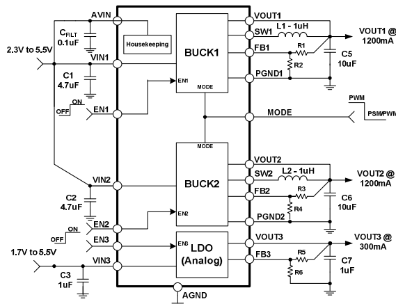
Figure 53. ADP5024 Adjustable Output Voltages with Enable Pins
