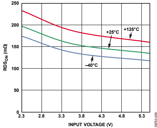
Figure 33. PMOS R_{DS(on)} vs. V_{IN}
