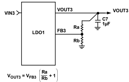
Figure 48. LDO1 External Output Voltage Setting
