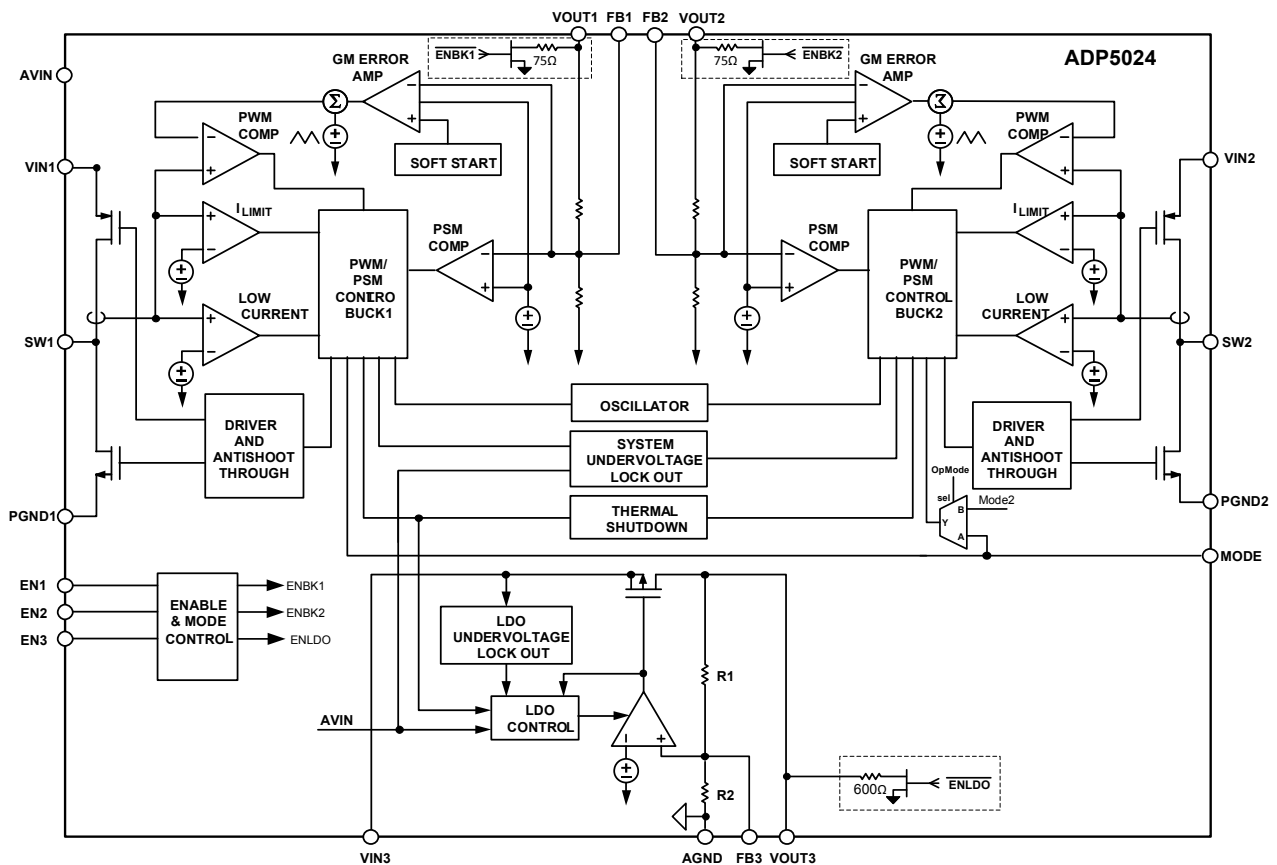
Figure 45. Functional Block Diagram
