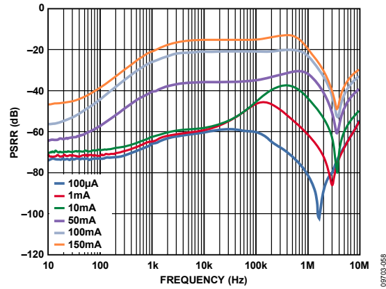
Figure 42. LDO PSRR Across Output Load, V_{IN3} = 3.3 V , V_{OUT3} = 3.0 V
