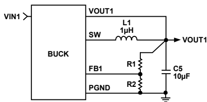
Figure 47. BUCK1 External Output Voltage Setting
