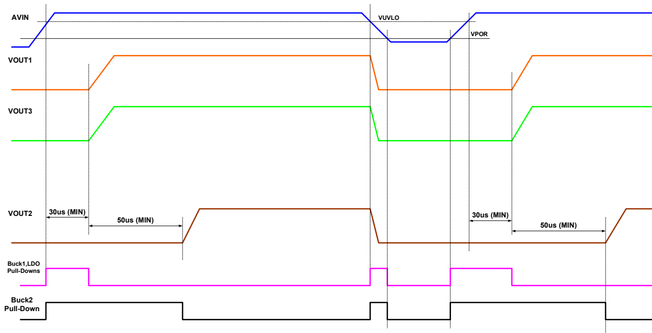
Figure 46. Regulator Sequencing on ADP5024 ( EN1 = EN2 = EN3 = V_{AVIN} )
