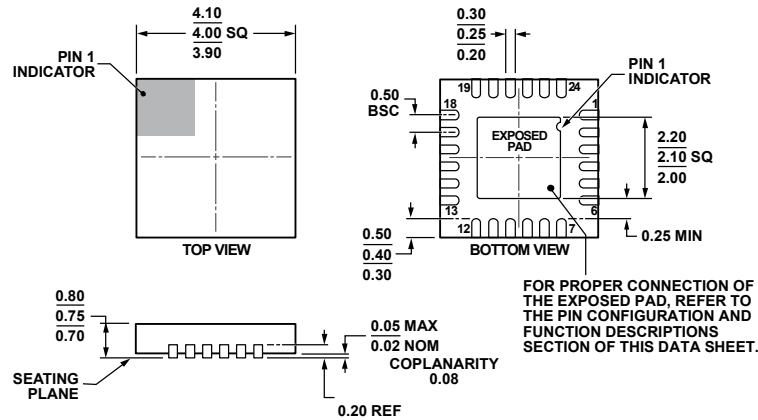
COMPLIANT TO JEDEC STANDARDS MO-220-WGGD-8. Figure 54. 24-Lead Lead Frame Chip Scale Package [LFCSP_WQ] 4 mm × 4 mm Body, Very Very Thin Quad (CP-24-10) Dimensions shown in millimeters
