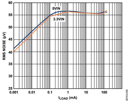
Figure 39. LDO Output Noise vs. Load Current, Across Input Voltage, V_{OUT3} = 2.8 V
