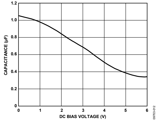
Figure 51. Capacitance vs. Voltage Characteristic
