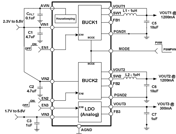
Figure 52. ADP5024 Fixed Output Voltages with Enable Pins
