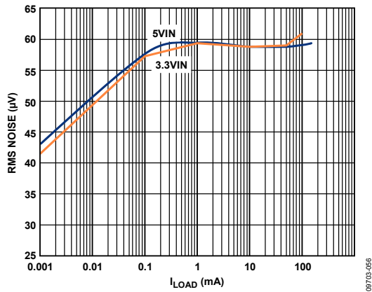
Figure 40. LDO Output Noise vs. Load Current, Across Input Voltage, V_{OUT3} = 3.0 V
