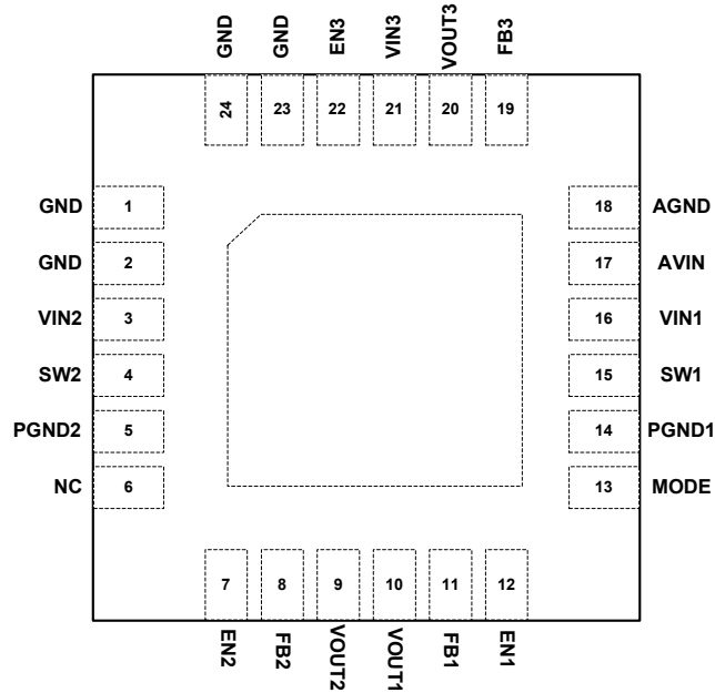
Figure 2. Pin Configuration—View from Top of the Die
