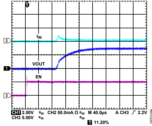
Figure 30. LDO Startup, V_{OUT3} = 3.0 V, I_{OUT3} = 5 mA
