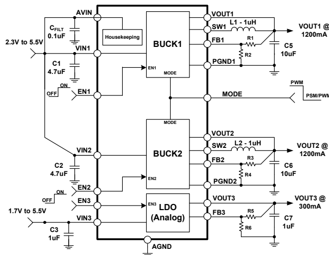
Figure 50. Processor System Power Management with PSM/PWM Control
