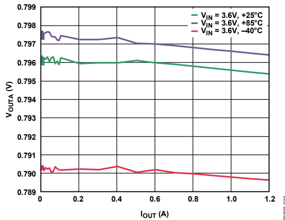
Figure 8. BUCK1 Load Regulation Across Input Voltage, V_{OUT1} = 3.3\text{ V} , PWM Mode
