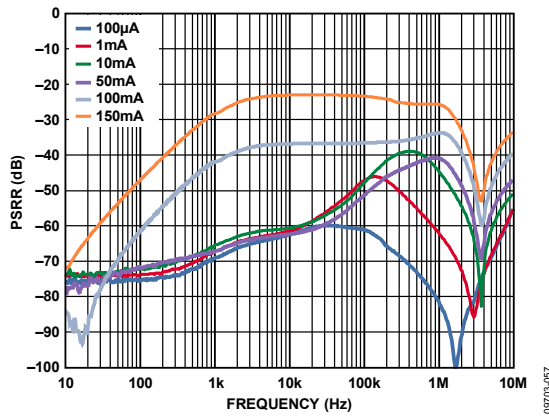
Figure 41. LDO PSRR Across Output Load, V_{IN3} = 3.3 V , V_{OUT3} = 2.8 V
