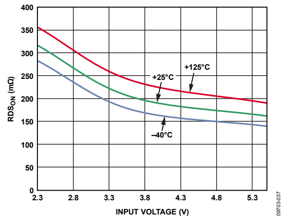
Figure 32. NMOS R_{DSon} vs. V_{IN}
