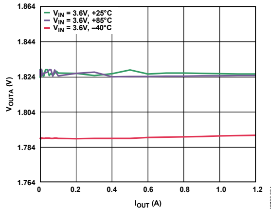
Figure 7. BUCK2 Load Regulation Across Temperature, V_{OUT2} = 1.8\text{ V} , Auto Mode
