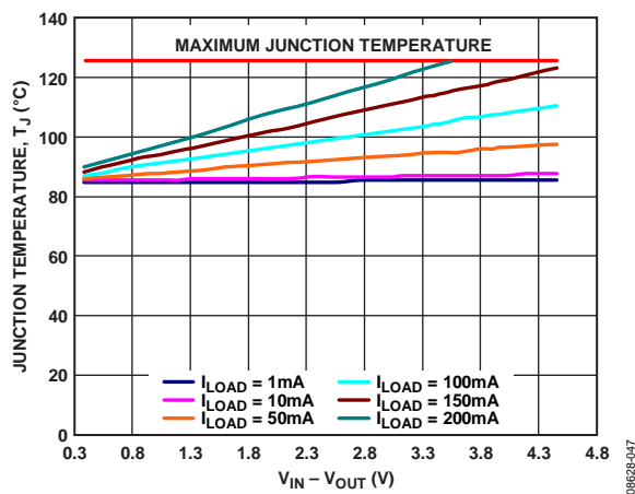
Figure 45. WLCSF, T_A = 85^\circ C
