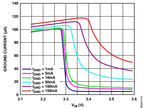
Figure 16. Ground Current vs. Input Voltage(VIN) in Dropout
