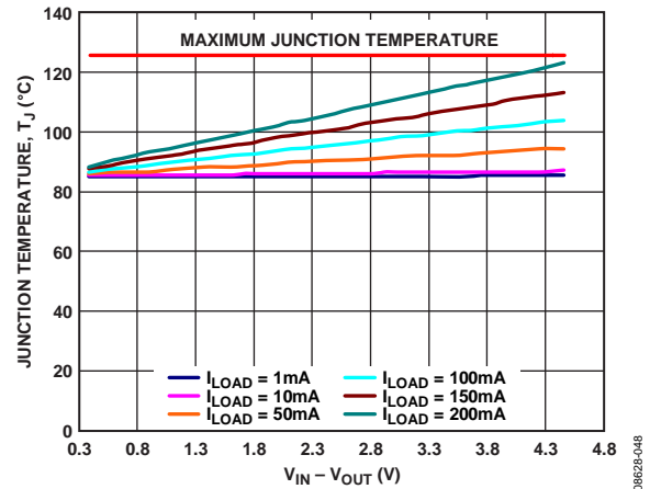
Figure 46. TSOT, T_A = 85^\circ C
