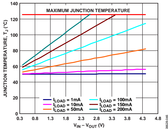
Figure 44. 100 mm 2 of PCB Copper, TSOT, T_A = 50^\circ C
