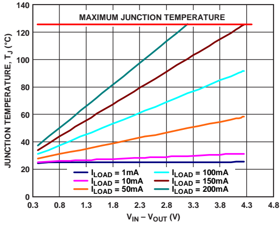
Figure 38. 100 mm 2 of PCB Copper, WLCSP, T_A = 50^\circ\text{C}
