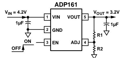
Figure 2. 5-Lead TSOT ADP161 with Adjustable Output Voltage, 3.2 V
