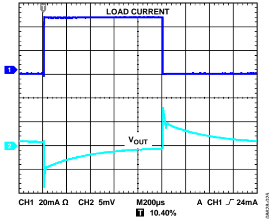
Figure 25. Load Transient Response, C_{IN}, C_{OUT} = 1 \mu F, I_{LOAD} = 1 \text{ mA to } 50 \text{ mA}, 200 \text{ ns Rise Time}, CH1 = \text{Load Current}, CH2 = V_{OUT}
