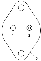
Pin 1 – Ground Pin 2 – V_{OUT} Case – V_{IN}
