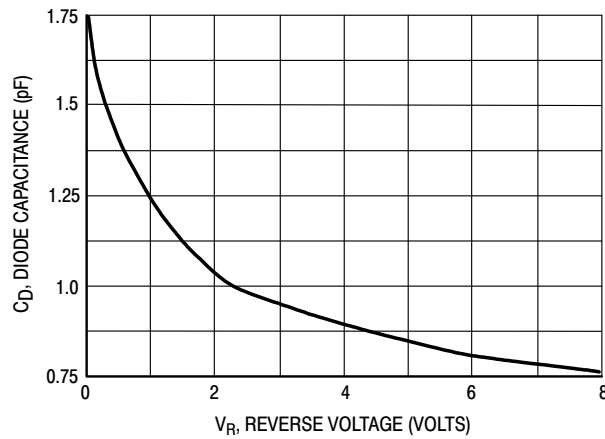
Figure 3. Diode Capacitance
