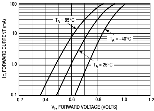
Figure 1. Forward Voltage
