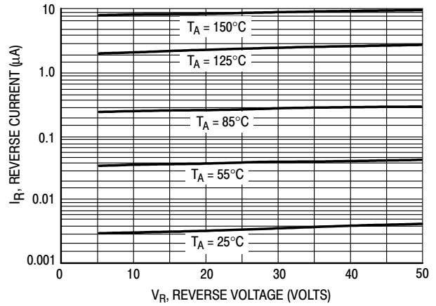
Figure 2. Reverse Current
