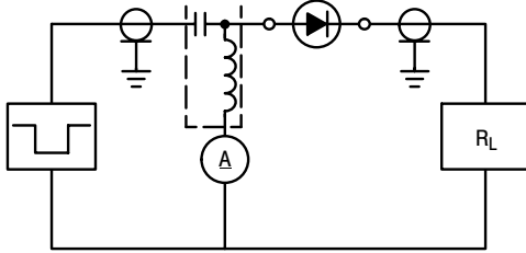
RECOVERY TIME EQUIVALENT TEST CIRCUIT
