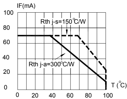
G.5 MAXIMUM FORWARD DC CURRENT VS TEMPERATURE. DERATING BASED ON T_{jmax}=110^{\circ} C
