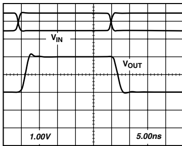
TPC 85. AD8130 Transient Response with +3\text{ V} Common-Mode Input
