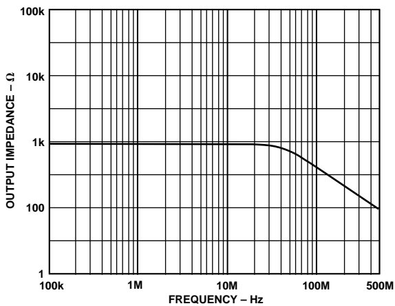
Figure 26. AD8109 Output Impedance, Disabled
