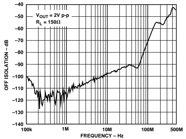
Figure 28. AD8109 Off Isolation, Input-Output
