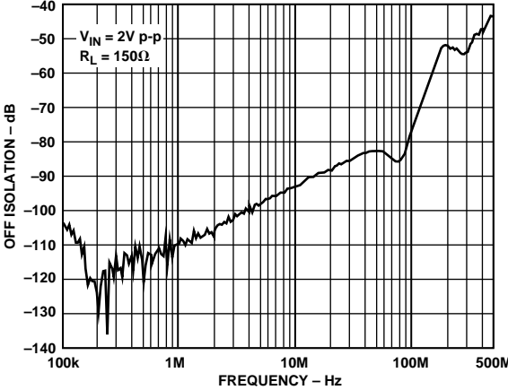
Figure 22. AD8108 Off Isolation, Input-Output
