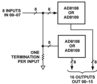
Figure 42. 8 \times 16 Crosspoint Array Using Two AD8108s (Unity Gain) or Two AD8109s (Gain-of-Two)
