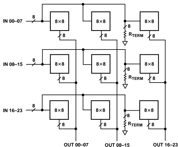
Figure 44. 24 \times 24 Crosspoint Array Using Nine AD8108s or AD8109s
