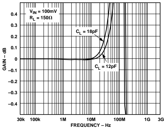
Figure 38. AD8109 Flatness vs. Capacitive Load
