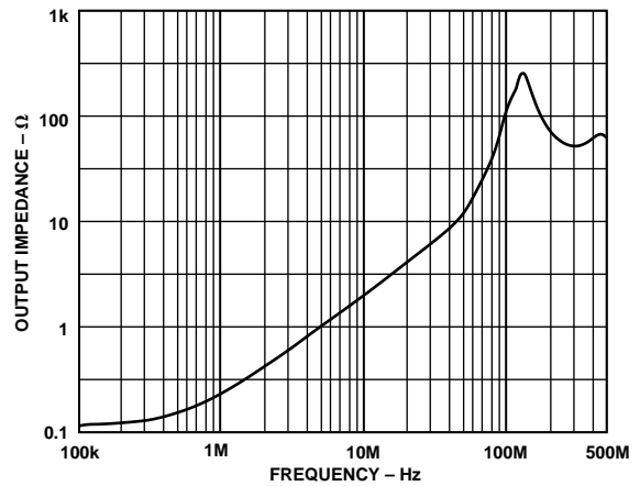
Figure 29. AD8109 Output Impedance, Enabled
