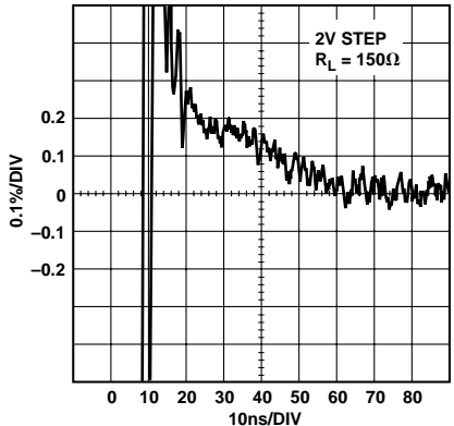
Figure 11. AD8108 Settling Time
