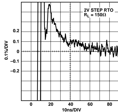
Figure 17. AD8109 Settling Time
