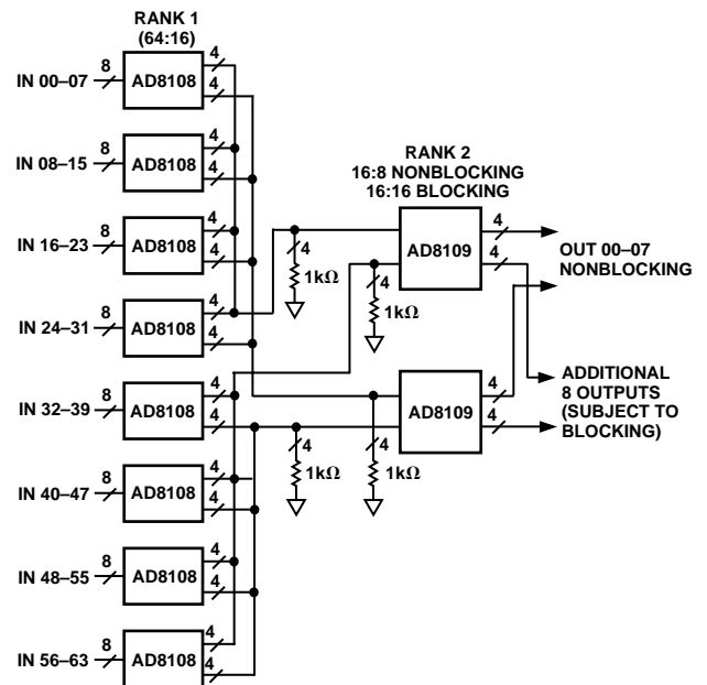
Figure 45. Nonblocking 64 \times 8 Array with Gain-of-Two ( 64 \times 16 Blocking)
