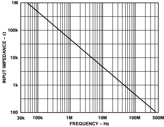
Figure 36. AD8109 Input Impedance vs. Frequency
