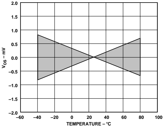
Figure 35. AD8108 Offset Voltage Drift vs. Temperature (Normalized at +25°C)
