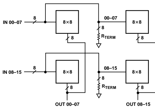
Figure 43. 16 \times 16 Crosspoint Array Using Four AD8108s or AD8109s
