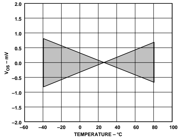
Figure 41. AD8109 Offset Voltage Drift vs. Temperature (Normalized at +25°C)
