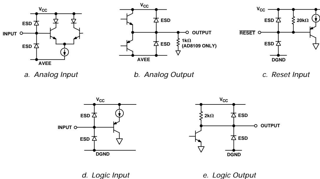
Figure 5. I/O Schematics
