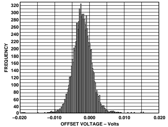
Figure 40. AD8109 Offset Voltage Distribution (RTI)
