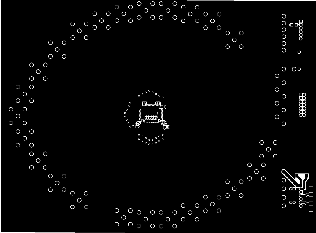
Figure 51. Board Layout (Bottom Layer)
