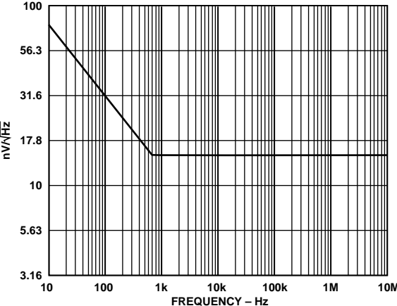
Figure 19. AD8108 Voltage Noise vs. Frequency
