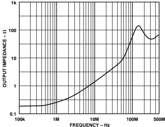
Figure 23. AD8108 Output Impedance, Enabled
