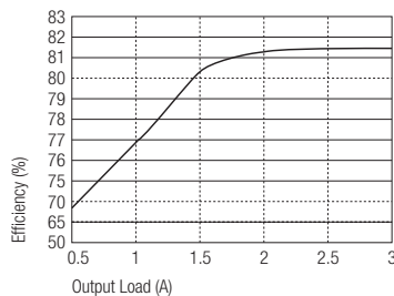
RP15-4805SEW Efficiency vs Output
