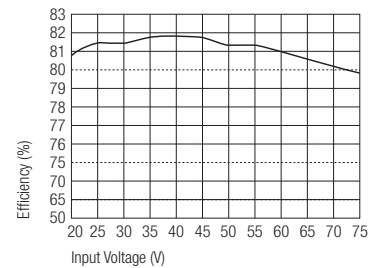
RP15-4805SEW Efficiency vs Input Voltage
