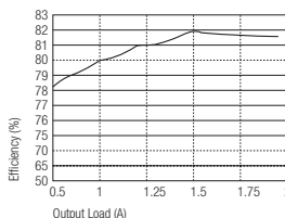
RP10-4805S Efficiency vs Output Load
