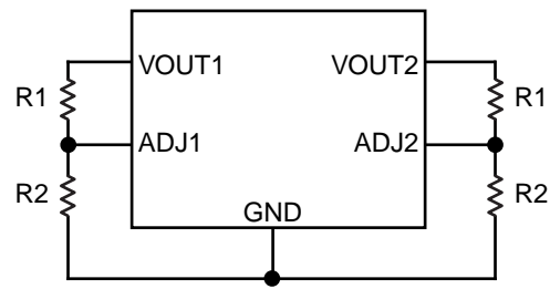
MIC2214 Adjustable Regulator Design
