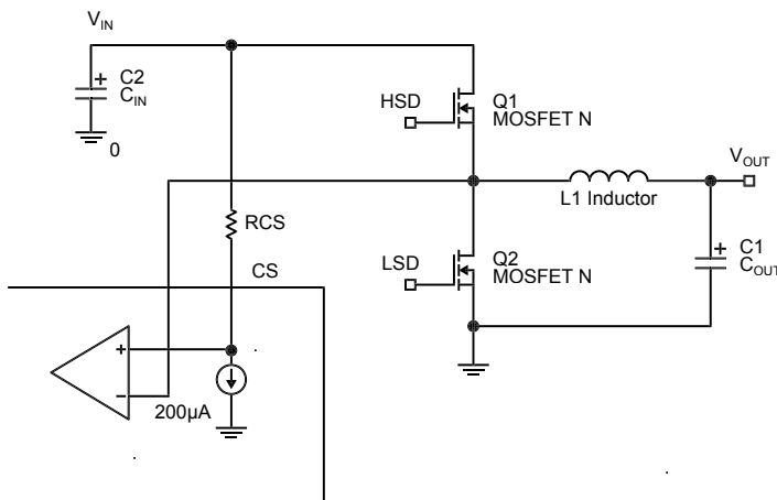
Figure 1. The MIC2168A Current Limiting Circuit
