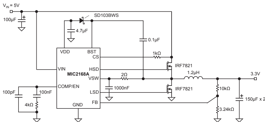
MIC2168A Adjustable Output 1MHz Converter
