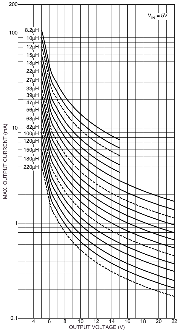
Figure7. Inductor Selection for V_{IN} = 5V
