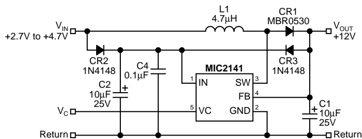
Figure 3. Bootstrap Configuration
