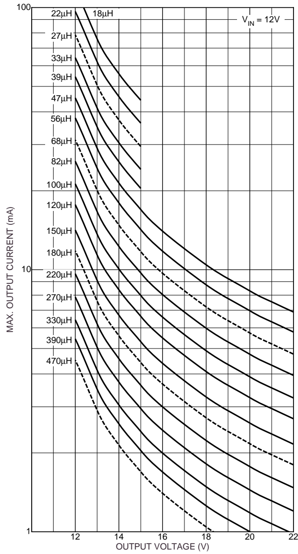
Figure 9. Inductor Selection for V_{IN} = 12V
