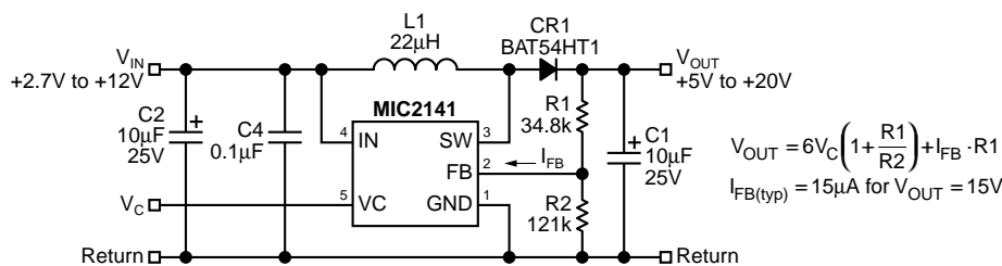
Figure 2. Gain-Boost Configuration
