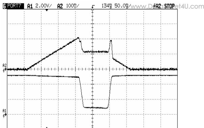
2009B SOT 502 #1 - Current ramp (5V) Radj=249ohms, Rfault=499ohms A1: Vout (2V/div) A2: Iout (500mA/div)
