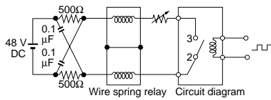
Circuit
