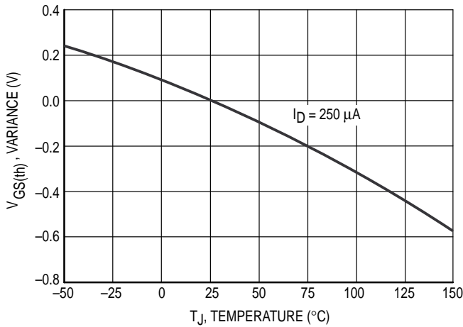
Figure 9. Threshold Voltage
