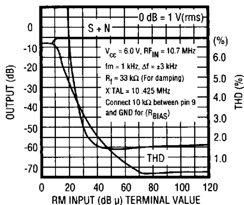
MIXER AND IF CHARACTERISTICS (10.7 MHz)
