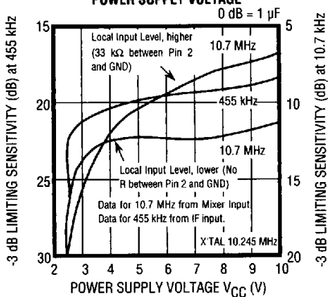
-3 dB LIMITING SENSITIVITY vs. POWER SUPPLY VOLTAGE
