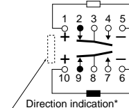
2-coil latching (Reset condition)
