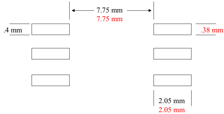
PCB pad for 32ld & 54ld SOIC Packages
