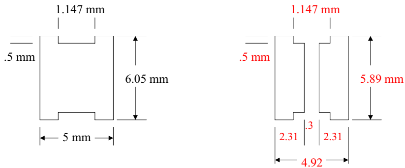
Figure 7. PCB Pad Dimensions for Lead of 32ld and 54ld SOICW & SOICW Packages
