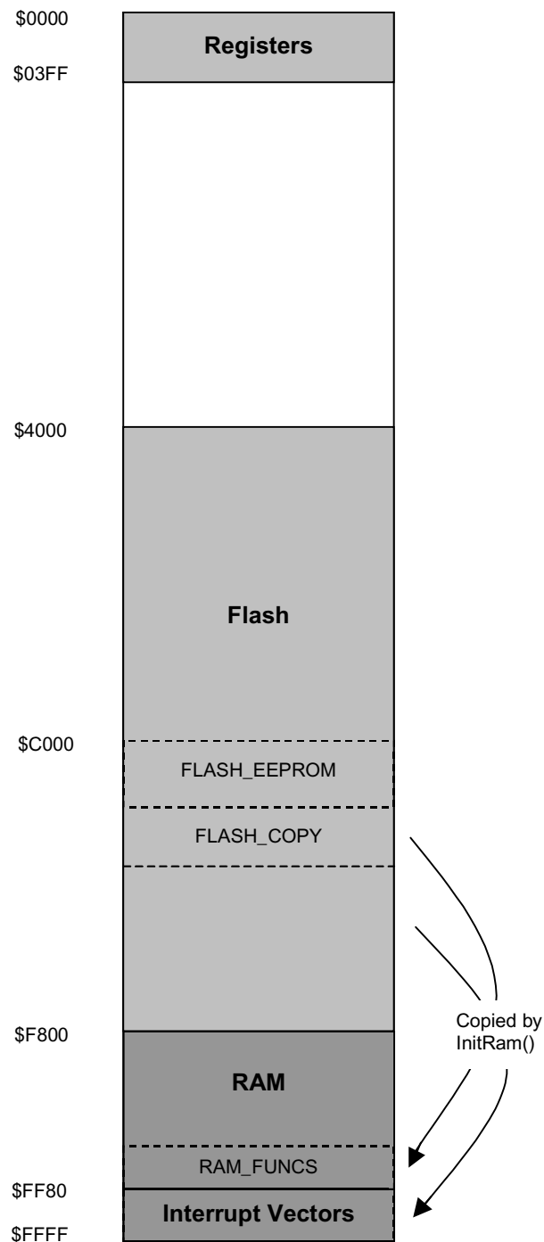
Figure 2. Example MC9S12C32 Memory Map with EEPROM Emulation and Interrupts
