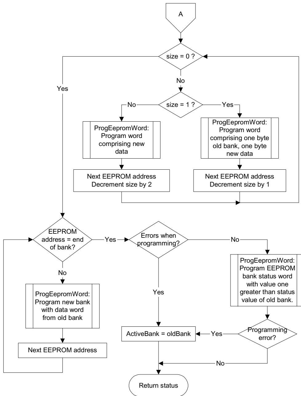
Figure 5. WriteEeprom Flow Diagram (continuation)
