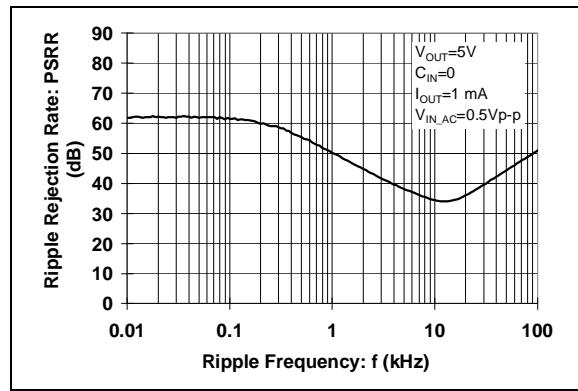
FIGURE 2-47: PSRR 5.0V @ 1 mA.
