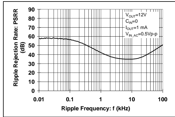
FIGURE 2-48: PSRR 12.0V @ 1 mA.
