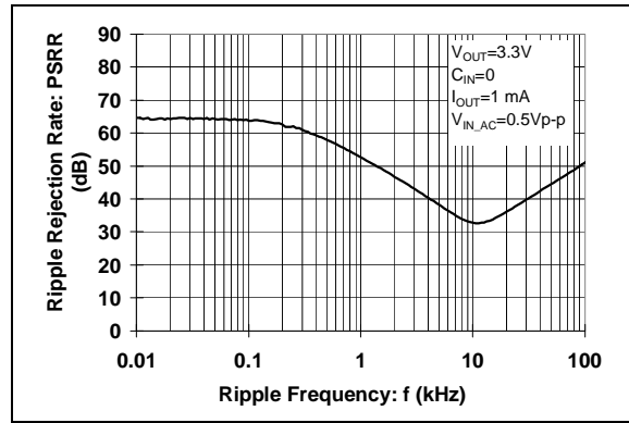
FIGURE 2-46: PSRR 3.3V @ 1 mA.
