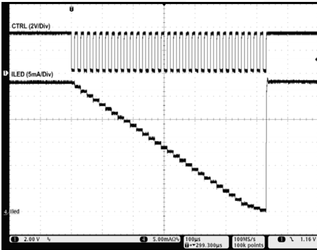
Figure 16. Dimming Operation
