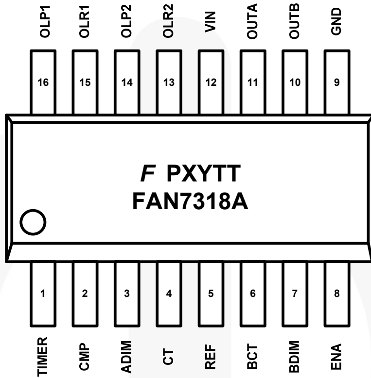
Figure 2. Package Diagram
