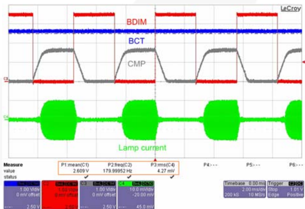
Figure 41. Negative Burst Dimming Waveform Using an External Pulse
