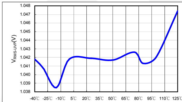
Figure 33. V_{RMS-UIVP} vs. Temperature
