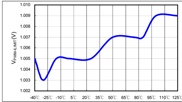
Figure 31. V_{PWM-ILIMIT} vs. Temperature
