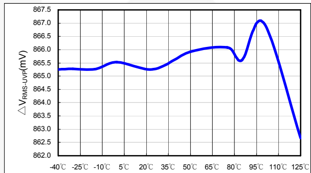
Figure 34. \Delta V_{RMS-UIVP} vs. Temperature
