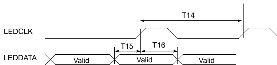
FIGURE 5. LED Interface
