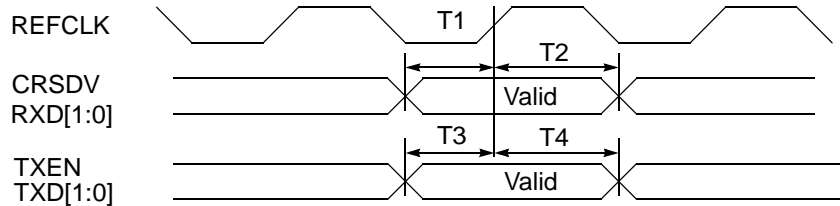
FIGURE 1. RMIi timing
