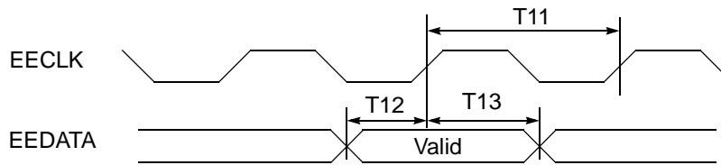
FIGURE 4. EEPROM timing
