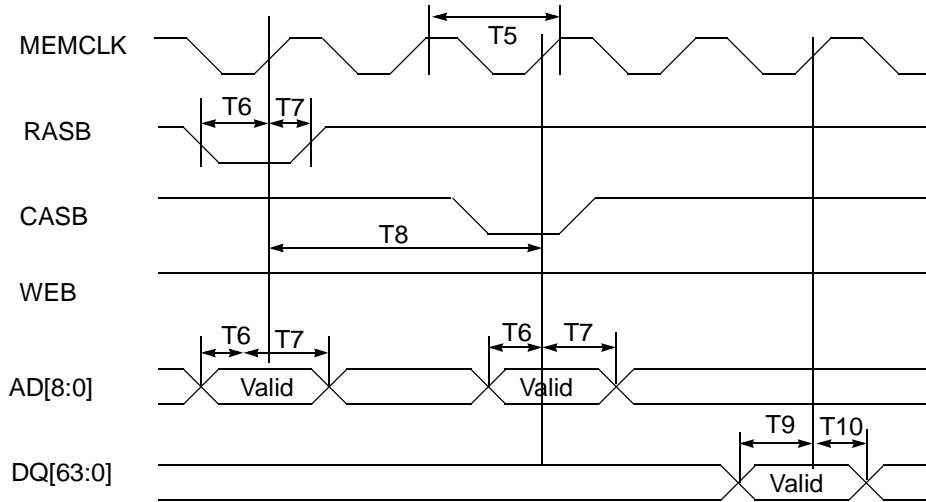
FIGURE 3. Memory Read Timing
