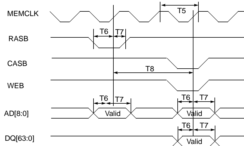
FIGURE 2. Memory Write Timing
