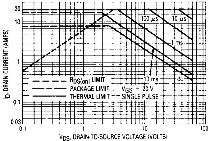
Figure 8. Maximum Rated Forward Biased Safe Operating Area
