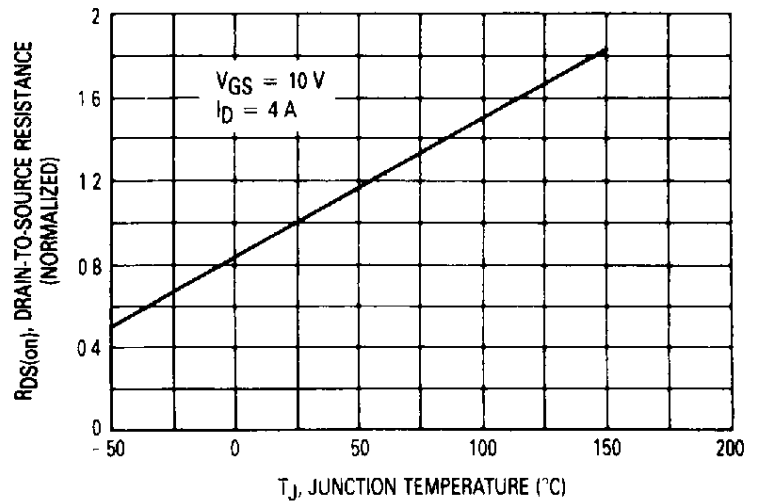
Figure 7. On-Resistance Variation With Temperature
