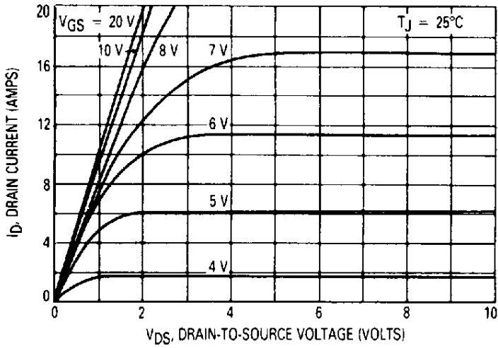
Figure 2. On-Region Characteristics
