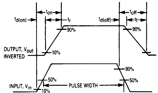
Figure 19. Switching Waveforms
