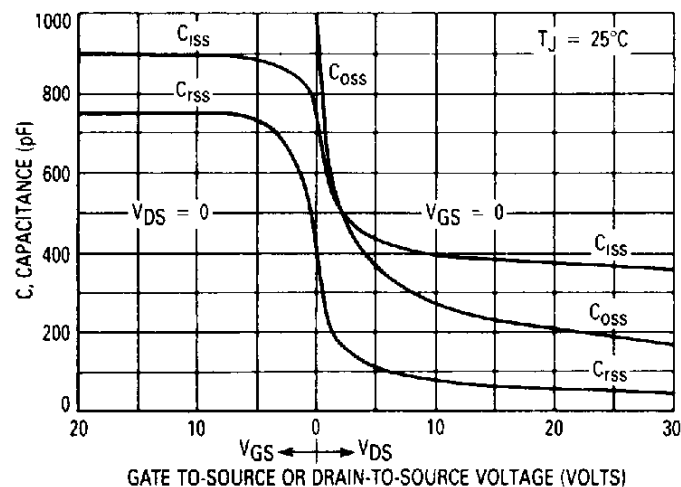
Figure 14. Capacitance Variation
