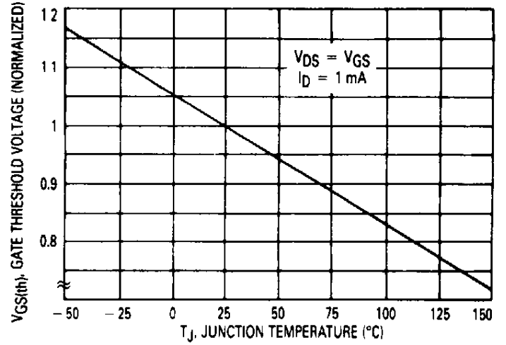
Figure 3. Gate-Threshold Voltage Variation With Temperature
