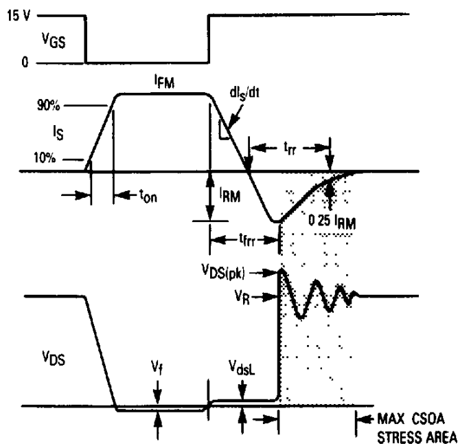
Figure 11. Commutating Waveforms
