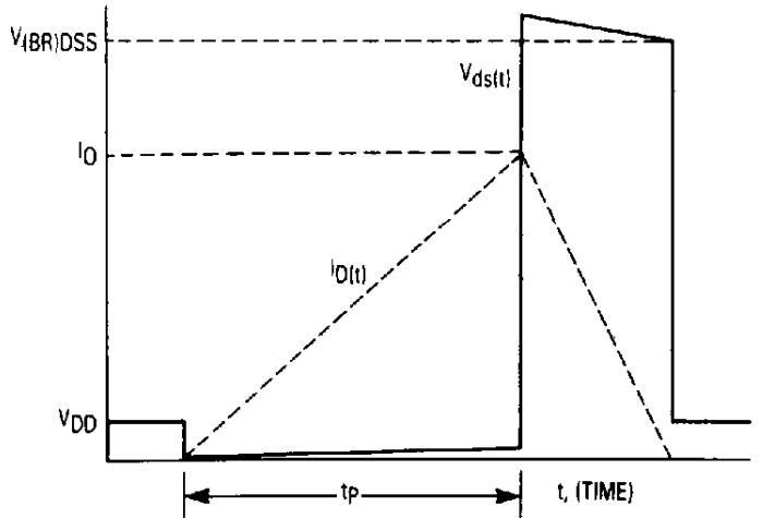
Figure 17. Unclamped Inductive Switching Waveforms
