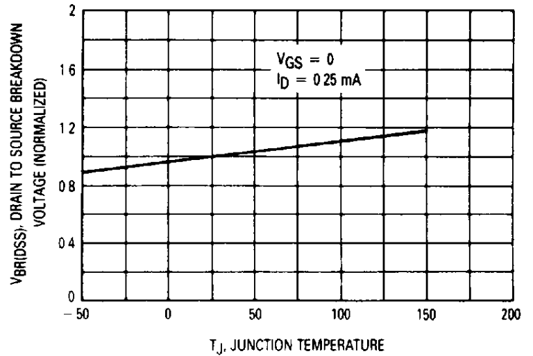
Figure 5. Breakdown Voltage Variation With Temperature
