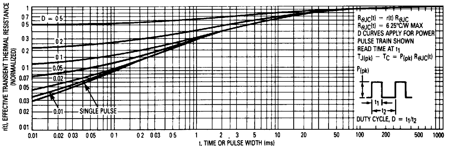
Figure 10. Thermal Response
