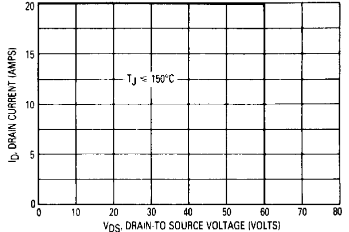
Figure 9. Maximum Rated Switching Safe Operating Area
