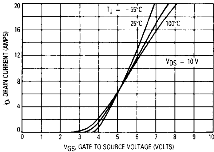
Figure 4. Transfer Characteristics
