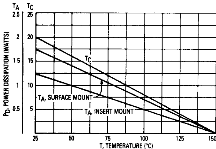
Figure 1. Power Derating
