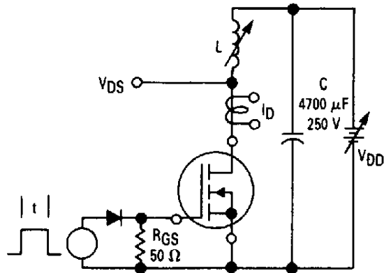
Figure 16. Unclamped Inductive Switching Test Circuit
