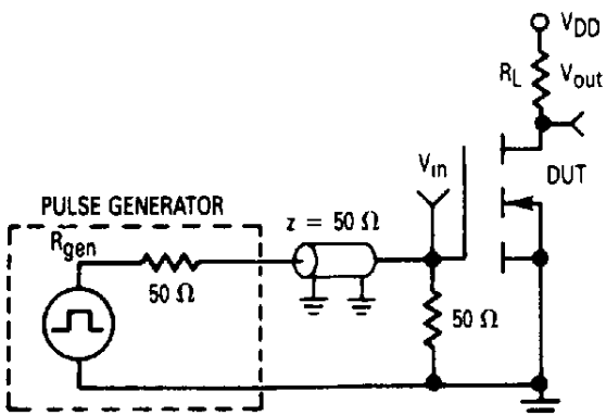
Figure 18. Switching Test Circuit
