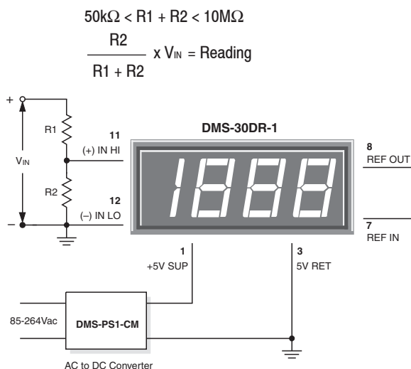
Figure 4. Input Attenuation Circuit
