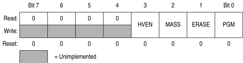
Figure 1. FLASH Control Register (FLxCR)
