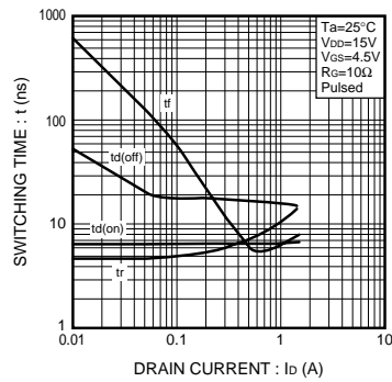
Fig.1 Switching Characteristics
