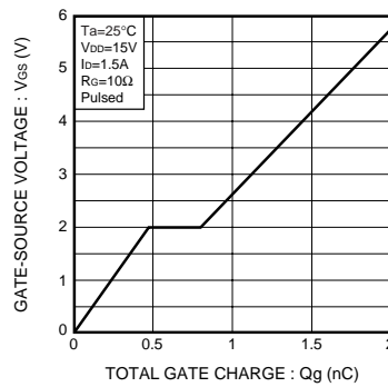
Fig.2 Dynamic Input Characteristics
