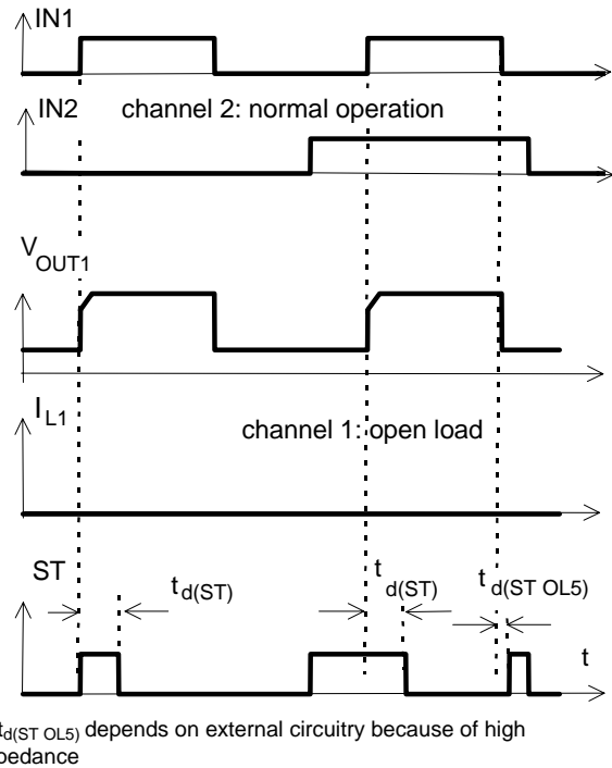
Figure 6a: Undervoltage:
