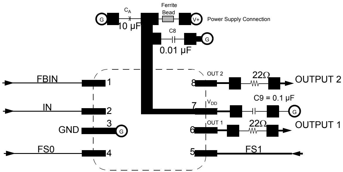
Figure 1. Schematic/Suggested Layout
