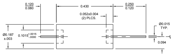
CASE STYLE M43
