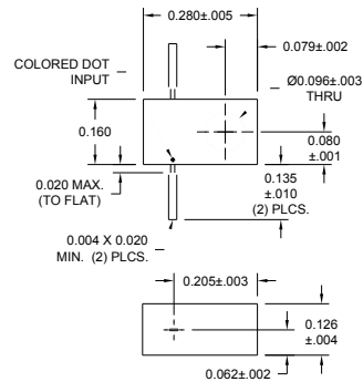
CASE STYLE M51
