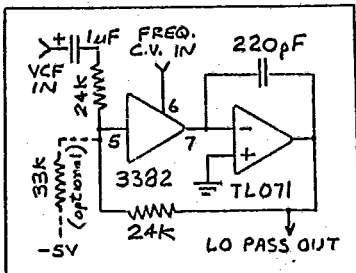
FIG. 2A: 3382 IN 1ST ORDER LOW PASS VCF
