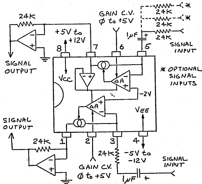
CEM3381/CEM3382 DUAL LOW NOISE VCA
