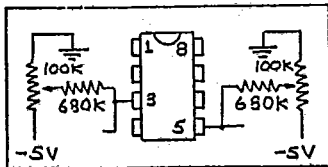
FIG. 1: 3381/3382 OPTIONAL FEEDTHROUGH TRIM
