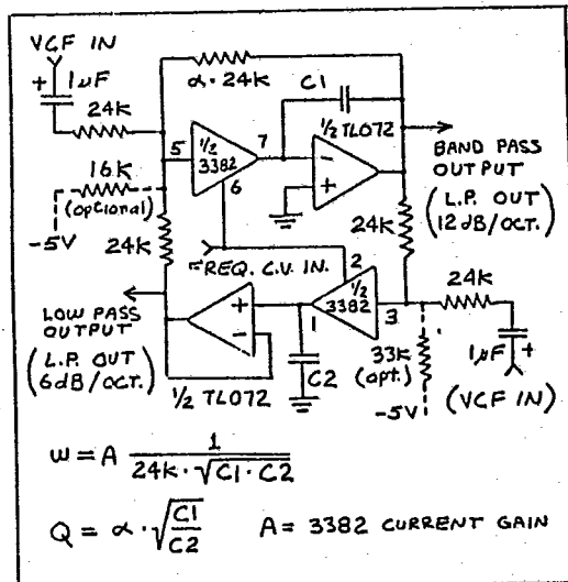
FIG. 2B: 3382 IN 2ND ORDER VCF
