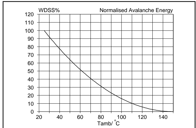
Fig. 15. Normalised avalanche energy rating. W_{DSS}\% = f(T_{amb}) ; conditions: I_D = 2.7\text{ A}
