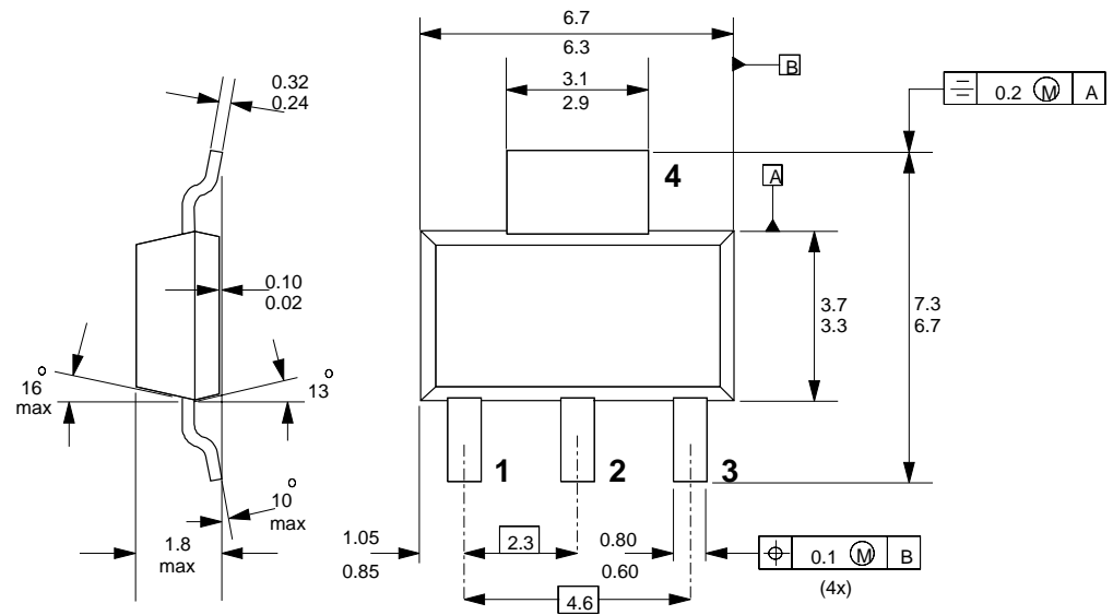
Fig.18. SOT223 surface mounting package.
