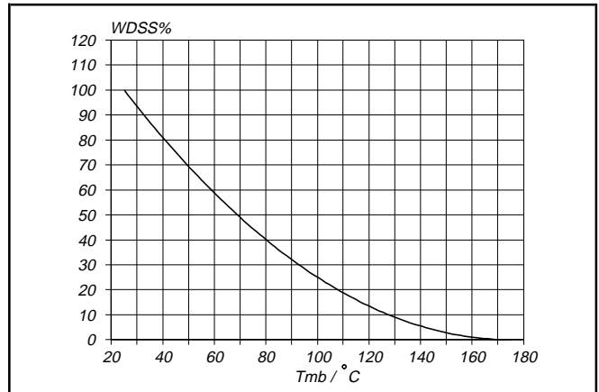
Fig. 15. Normalised avalanche energy rating. W_{DSS}\% = f(T_{mb}) ; conditions: I_D = 50 A
