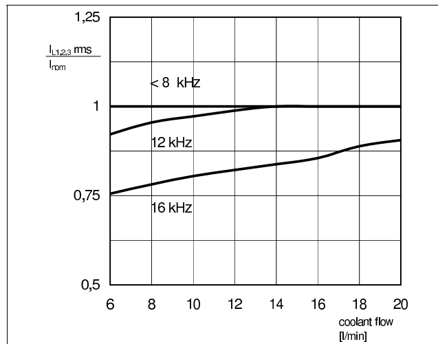
Fig. 4: Normalized output current vs. coolant flow
