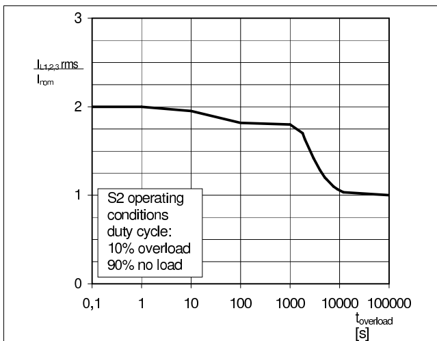
Fig. 5: Overload capability
