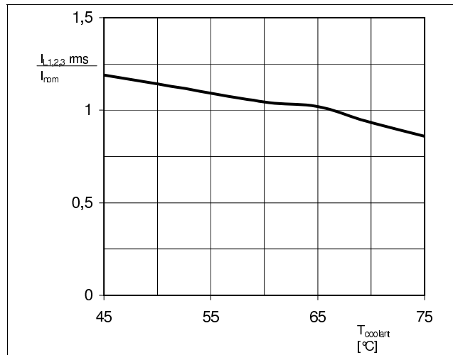
Fig. 2: Normalized output current vs. coolant temperature
