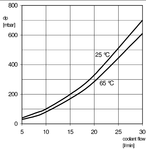
Fig. 7: Pressure drop characteristic
